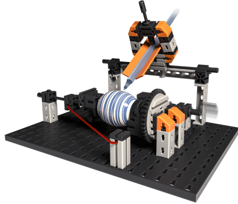
Yumurta Boyama Makinesi / Egg painting machine/ Machine ..... 11
